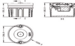
CM-HT12/D aim point landing light
